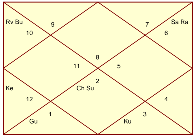
Dwadasamsa - Parents
