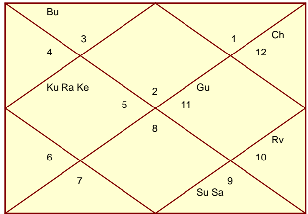
Vimsamsa - Vehicle
