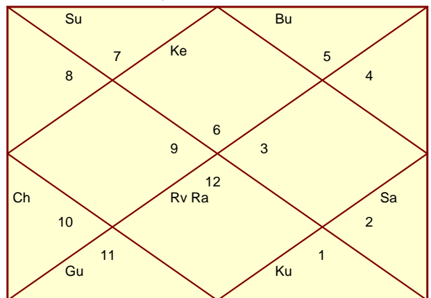
Sapthamsa - Issues
