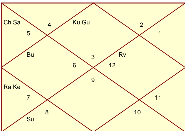
Sasthamsa - Health
