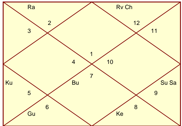
Panchamsa - Spiritual
