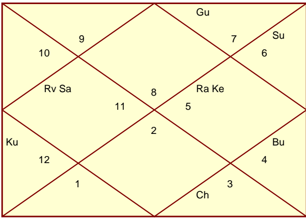
Ashtamsa - Longevity
