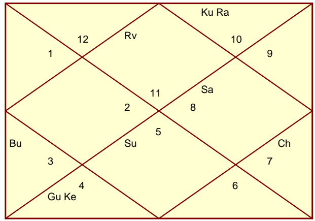
Navamsa - Spouse
