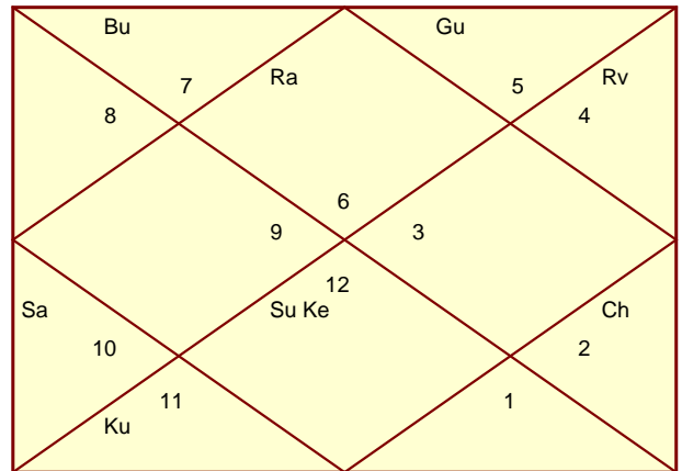
Shashtyamsa - All
